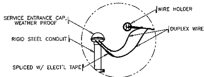
DETAIL "B"
